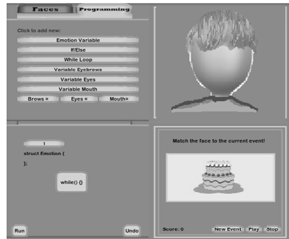
Figure 1. The visual drag-and-drop programming interface which allows the user to manipulate the virtual character's facial expressions.
